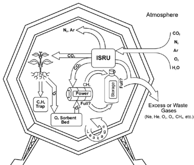
Figure 9: MDG Gas Cycle
