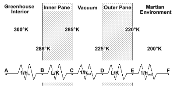
Figure 12: Diagram of thermal upper hemisphere heat loss used in determining radiative balance.
