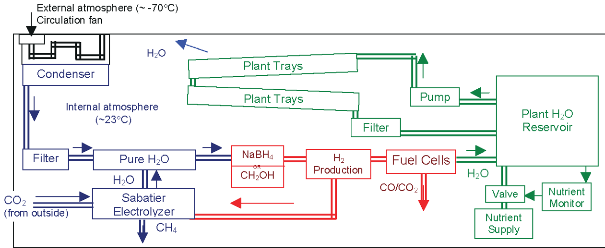
Figure 7: MDG Water Flow
